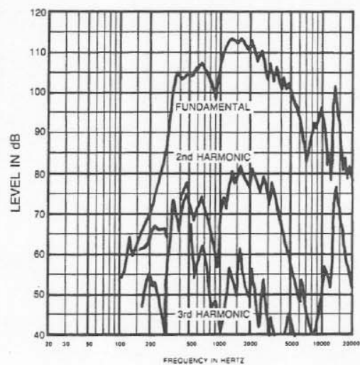
FIGURE 3 CFID32 Frequency Response (1 watt at 1 meter)
