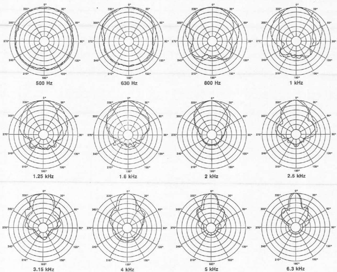
FIGURE 1 CFID32 Polar Response
