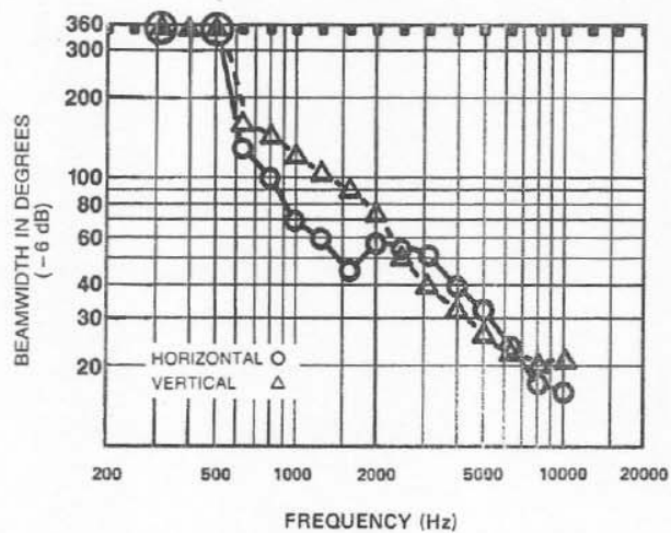
FIGURE 2 CFID32 Polar Response
